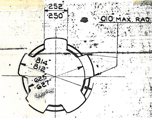
VIEW SHOWING FORM OF 5 EQUISPACED SPLINES
